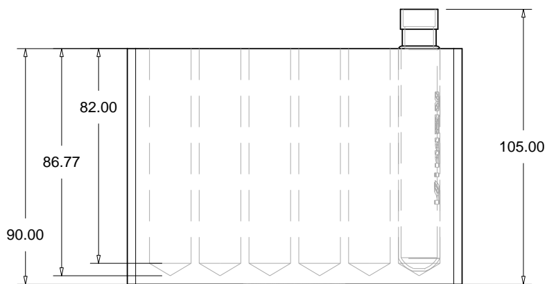
Heat Block with KIMAX ® Culture Tube 16x100, 12 ml
